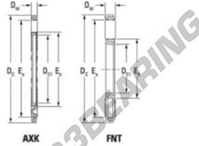
Boundary dimensions
