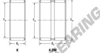
Basic needle roller and cage assemblies
