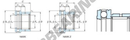
Boundary dimensions
