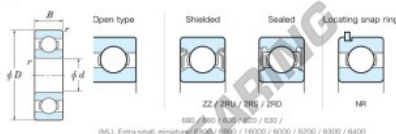
Boundary dimensions
