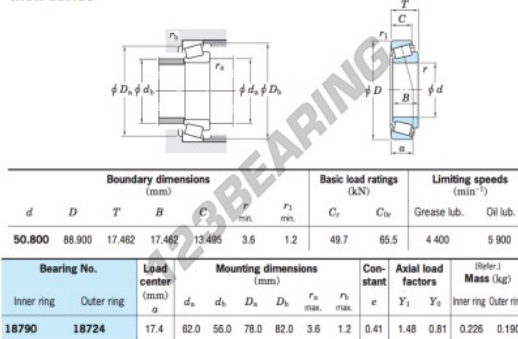
Single-row tapered roller bearings inch series Koyo
