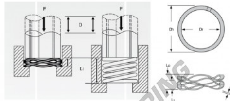
Multispring Compression Rings
